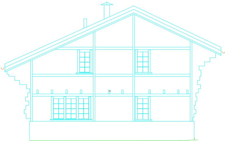
South Elevation
